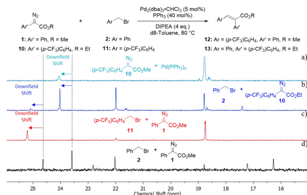
Fig. 6 ^{31}\text{P}\{^1\text{H}\} NMR (243 MHz) at 80 °C in \text{d}_8 -toluene. Comparison of ^{31}\text{P} spectra of differing starting materials. a) 10 and \text{Pd}_2(\text{dba})_3\cdot\text{CHCl}_3/\text{PPh}_3 ; b) in situ reaction of 2 and 10 substrates; c) in situ reaction of 11 and 1 substrates; d) in situ model reaction. Reaction conditions [\mathbf{2}]/[\mathbf{11}] 0.1 M, [\mathbf{1}]/[\mathbf{10}] 0.3 M, [\text{DIPEA}] 0.4 M, [\text{Pd}] 0.01 M, [\text{PPh}_3] 0.04 M, \text{d}_8 -toluene (0.6 mL), 80 °C.
