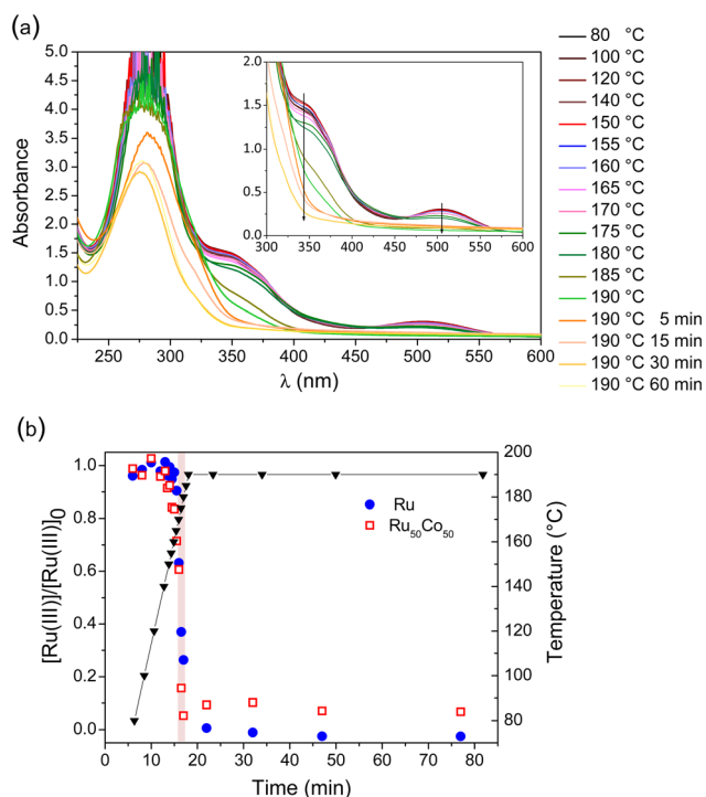
Fig. 2 (a) UV-visible spectra obtained during heating an equimolar solution of \text{Ru(acac)}_3 and \text{Co(acac)}_2 in octan-1-ol. Inset: Magnification in the 300–600 nm range. (b) Evolution of the relative \text{Ru(III)} concentration during the synthesis of Ru (●) and \text{Co}_{50}\text{Ru}_{50} (□) NPs deduced from the absorbance value at 506 nm and associated temperatures (▼) at which the aliquots were taken.
