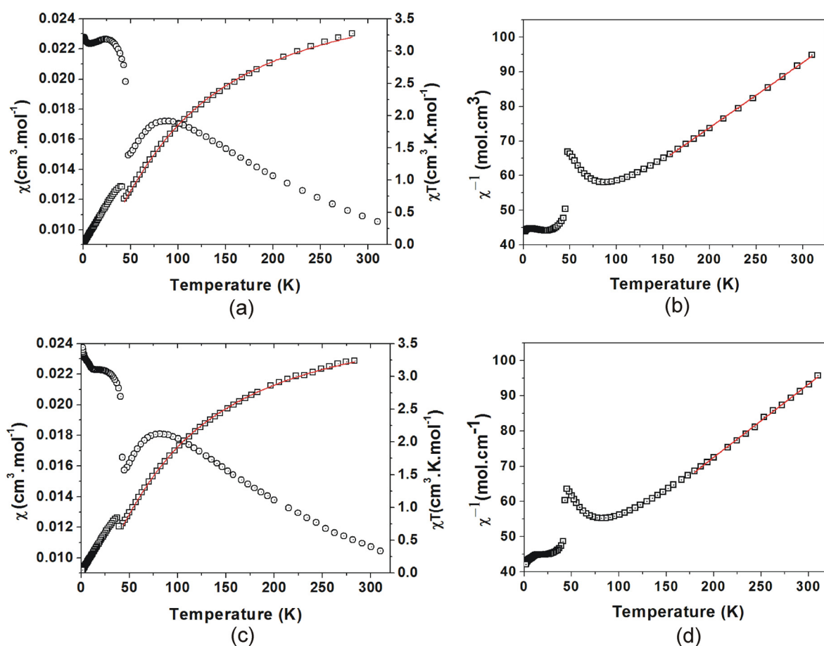
Fig. 13 (a) \chi(T) (□) and \chi T(T) (○) plots for C4MnCl between 1.8 K and 310 K. The red line through the data points corresponds to the fit of the S = 5/2 AFM square lattice model from T_N to 310 K. (b) \chi^{-1}(T) plot for C4MnCl between 1.8 K and 310 K. The red line through the data points corresponds to a linear fit between 157 K and 310 K. (c) \chi(T) (□) and \chi T(T) (○) plots for C6MnCl between 1.8 K and 310 K. The red line through the data points corresponds to the fit of the S = 5/2 AFM square lattice model from T_N to 310 K. (d) \chi^{-1}(T) plot for C6MnCl between 1.8 K and 310 K. The red line through the data points corresponds to a linear fit between 180 K and 310 K.
