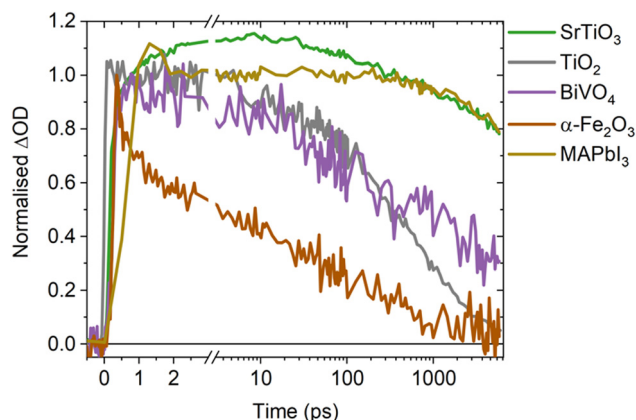
Fig. 4 Comparison of the decay kinetics of SrTiO 3 to other metal oxides (anatase TiO 2 , BiVO 4 and \alpha -Fe 2 O 3 , at photogenerated charge densities of 10 18 cm -3 ) and MAPbI 3 (at a photogenerated charge density of 10 17 cm -3 ).
