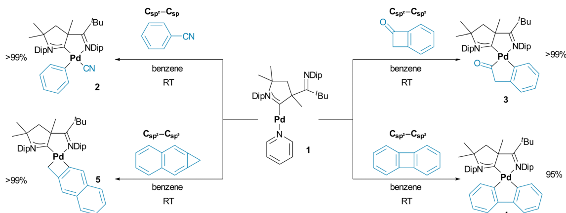
Scheme 2 Insertion of complex 1 into C sp 2 –C sp , C sp 2 –C sp 2 and C sp 2 –C sp 3 bonds.
