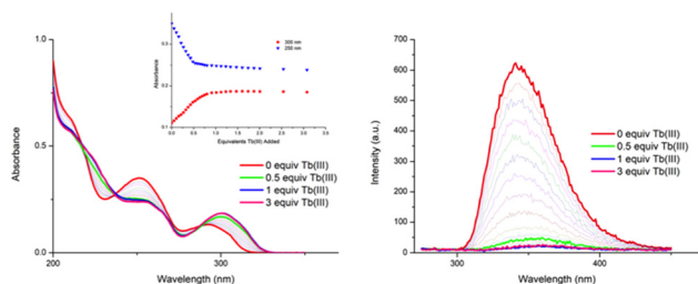
Fig. 2 The overall changes in the (left) UV-visible absorption spectra and (right) fluorescence emission spectra ( \lambda_{exc} = 260 nm) upon titrating 1 ( 1 \times 10^{-5} M) against Tb(CF_3SO_3)_3 (0 → 3 equiv.) in CH_3CN at 22 °C. Inset: The binding isotherms of absorbance at \lambda = 300 and 250 nm, respectively.
