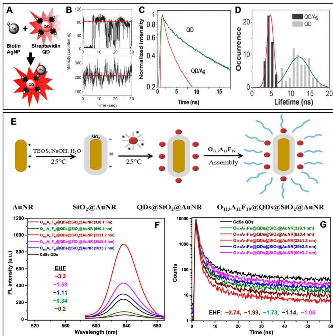
Fig. 10 Examples of solution-based metal–QD nanostructures for PEF. (A) Schematic of a solution-based nanostructure consisting of streptavidin-coated QDs and biotinylated AgNPs. (B) Typical intensity trajectories from a single QD (top) or single QD/Ag nanocomposite (bottom) on glass substrates. The red dotted lines present the maximum occurrence of single QD intensities, which is circa 2.6-fold higher for the QD/Ag nanohybrids. (C) PL decays of QD and QD/Ag nanohybrids. (D) On average, single QD/Ag nanohybrids showed a circa 2.6-fold faster PL lifetime compared to bare QDs. All experiments were performed with \lambda_{\text{ex}} = 470 nm and \lambda_{\text{em}} = 655 \pm 10 nm. A to D adapted with permission from ref. 134. Copyright 2009 The Royal Society of Chemistry. (E) Fabrication procedure of aqueous metal–QD nanostructures consisting of SiO 2 -coated AuNRs, CdSe QDs, and a co-block polymer coating (O 113 A 11 F 19 ) corresponds to the polymerization degree of blocks O, A, and F. (F) PL spectra ( \lambda_{\text{ex}} = 520 nm) of bare QDs and QD/AuNR nanohybrids with different SiO 2 shell thicknesses. EHF correspond to the ratios of QD/AuNR and bare QD PL intensities. (G) PL decay curves ( \lambda_{\text{ex}} = 520 nm) of bare QDs and QD/AuNR nanohybrids with different SiO 2 shell thicknesses. EHF correspond to the ratios of bare QD and QD/AuNR PL lifetimes. E to G adapted with permission from ref. 135. Copyright 2021 Elsevier B.V.
