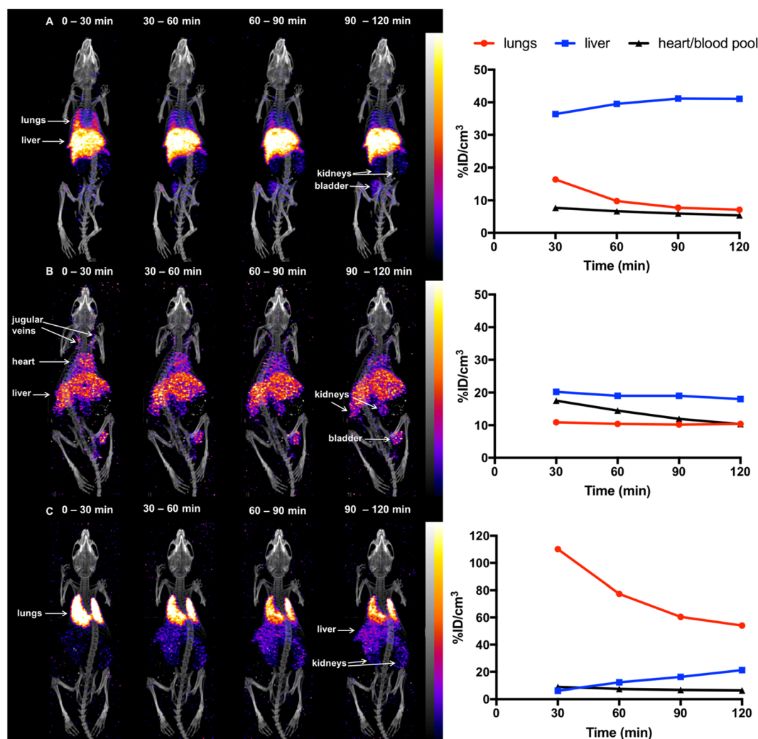
Fig. 3 SPECT/CT maximum intensity projections and ^{111}\text{In} concentrations in specific organs for mice administered (a) [ ^{111}\text{In} ]In-DTPA-CTP-labelled 5T33 cells (SPECT scale of 0.8–8 \% \text{ID g}^{-1} ), (b) [ ^{111}\text{In} ]In-DTPA-CTP (cell-free) (SPECT scale of 1.6–8 \% \text{ID g}^{-1} ) and (c) [ ^{111}\text{In} ]In-(oxine) 3 -labelled 5T33 cells (SPECT scale of 1.6–16 \% \text{ID g}^{-1} ), acquired 0–30 min, 30–60 min, 60–90 min and 90–120 min post-injection.
