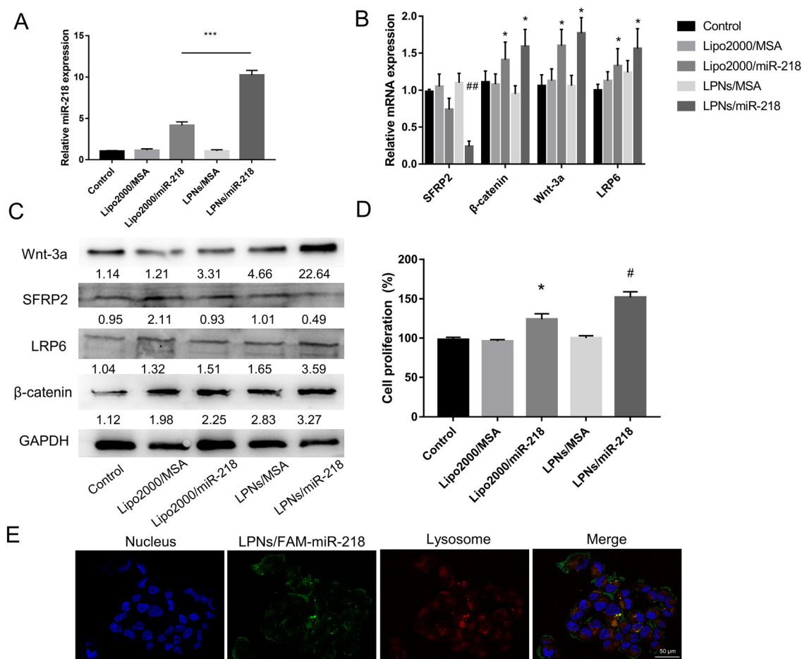
Fig. 2 Intracellular uptakes of LPNs/miR-218. The mRNA level of mature miR-218 (A), mRNA (B), and protein (C) levels of Wnt-3a, \beta -catenin, LRP6, and SFRP2 in DP cells after transfection, *** P < 0.005 and ## P < 0.01 vs. Lipo2000/miR-218, * P < 0.05 vs. Control. (D) The cell proliferation of DP cells after different transfection, * P < 0.05 vs. Control and # P < 0.05 vs. Lipo2000/miR-218. (E) Confocal laser microscope (CLSM) images of cells treated with LPNs/FAM-miR-218 for 4 h (blue = nuclei; red = lysosomes, stained with LysoTracker Red; green = FAM-miR-218, scale bars = 50 \mu m). Data were shown as mean \pm SD ( n = 5 ), and statistical significance was calculated by one-way ANOVA followed by Dunnett's test.
