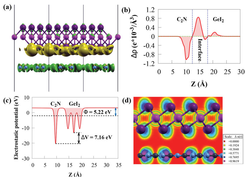
Fig. 4 (a) Three-dimensional charge density difference of the GeI 2 /C 2 N vdW heterostructure with an iso-value of 0.0008 \text{ e bohr}^{-3} . Green and yellow isosurfaces denote charge depletion and accumulation, respectively. (b) The averaged difference in the electron density for the GeI 2 /C 2 N vdW heterostructure along the z-axis. The inner surfaces of the two materials are marked with a blue dashed line. (c) The potential drop ( \Delta V ) for the GeI 2 /C 2 N vdW heterostructure. (d) Electron localisation functions across the GeI 2 /C 2 N vdW heterostructure interface. Grey, blue, magenta and purple balls denote C, N, Ge and I atoms, respectively.
