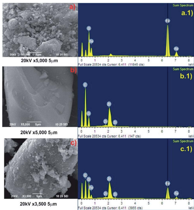
Fig. 1 SEM micrographs and EDAX analysis of (a) \text{Fe}_3\text{O}_4 ; (b) Zr-MOF; (c) Zr-MOF@ \text{Fe}_3\text{O}_4 .
