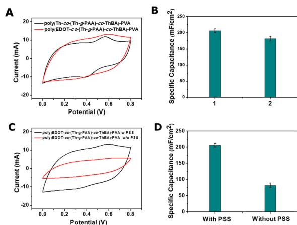
Fig. 2 (A) Cyclic voltammograms (CVs) and (B) areal specific capacitances of (1) poly(EDOT- co -(Th- g -PAA)- co -ThBA)-PVA hydrogels and (2) poly(Th- co -(Th- g -PAA)- co -ThBA)-PVA hydrogel electrodes in 2 M KCl solution at a scan rate of 100 mV s -1 . (C) CV and (D) areal specific capacitance of poly(EDOT- co -(Th- g -PAA)- co -ThBA)-PVA hydrogels with and without PSS.
