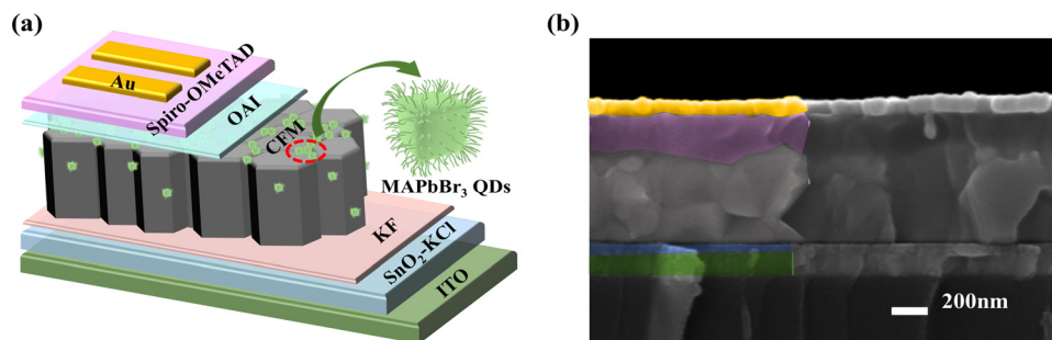
Fig. 1 (a) Device structure diagram and (b) cross-sectional SEM images of the PSCs.
