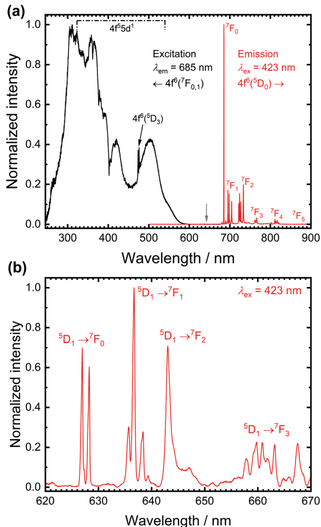
Fig. 1 (a) Photoluminescence excitation (black, \lambda_{em} = 685 \text{ nm} ) and emission (red, \lambda_{ex} = 423 \text{ nm} ) spectrum of \text{SrB}_4\text{O}_7:0.5\% \text{Sm}^{2+} at room temperature. The emission lines are assigned to the ^5\text{D}_0 \rightarrow ^7\text{F}_J ( J = 0 \dots 6 ) transitions of \text{Sm}^{2+} . (b) High-resolution spectrum in the spectral range marked with the grey arrow in (a) indicates the presence of weak ^5\text{D}_1 \rightarrow ^7\text{F}_J transitions.
