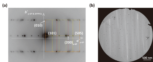
Fig. 4 (a) SAED patterns (a) and the corresponding electron micrograph (b) of 2FPICz thin films deposited on the p -6P double-layer. The red and yellow dashed grids represent the crystal lattices of p -6P and 2FPICz, respectively.
