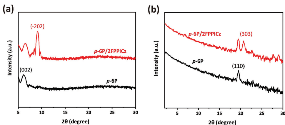
Fig. 3 (a) Out-of-plane and (b) in-plane XRD patterns of double-layer p -6P and 20 nm WEG 2FPICz crystalline thin films.
