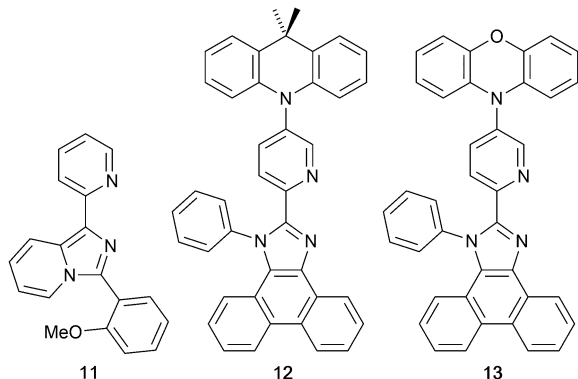
Scheme 7 Structures of imidazolyl pyridine derivatives used in [Cu(P ^ AP)-(N ^ N)] + complexes.
