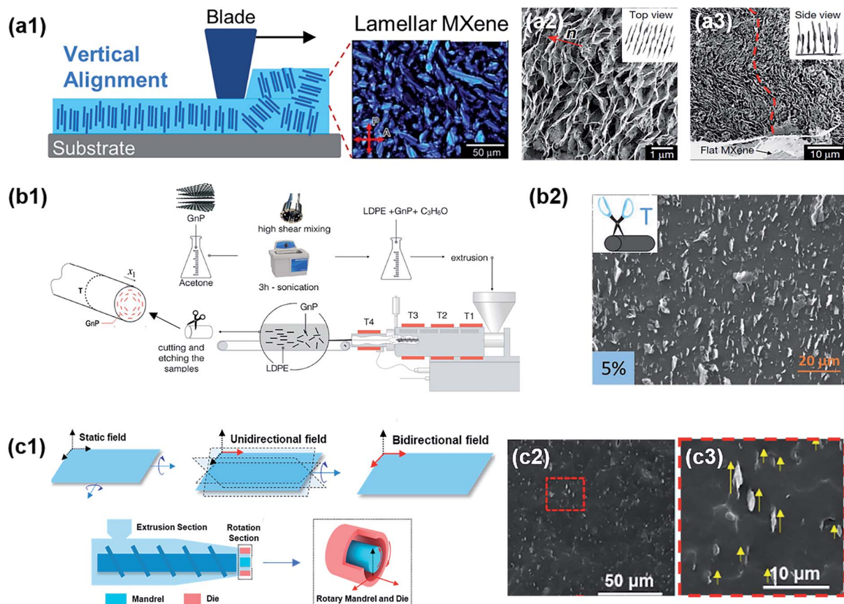
Fig. 10 Vertical alignment of 2D nanomaterials assisted by shear force. (a1) Schematic representation of tape casting of liquid-crystalline Ti_3C_2T_x . Reproduced from ref. 185 with permission from Elsevier. (a2) Top view SEM image of the MXene lamellar liquid crystal (MXLLC). (a3) Side view of vertical MXene nanosheets. Reproduced from ref. 116 with permission from Springer Nature. (b1) Schematic representation of the extrusion process of graphite nanoplatelet (GNP) and polyethylene (LDPE) nanocomposites. (b2) Surface morphology of the extruded GNP–LDPE composite with the transverse section. Reproduced from ref. 183 with permission from John Wiley and Sons. (c1) Schematic illumination of the rotation extrusion equipment. (c2) Cross-sectional SEM images of the extruded composites. (c3) Magnified area of (c2) in which yellow arrows refer to the nanofiller alignment direction. Reproduced from ref. 184 with permission from Elsevier.
