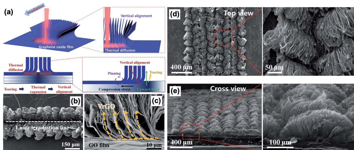
Fig. 11 Vertical alignment of reduced graphene oxide nanosheets by laser irradiation. (a) Schematic of the CO_2 laser irradiation fabrication process of the vertically aligned nanostructure. (b and d) Top view of the vertically aligned nanosheets. (c and e) Cross-sectional view of the as-fabricated nanostructure. Reproduced from ref. 186 with permission from Elsevier.
