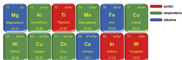
Fig. 1 Acidity and alkalinity of metal oxides.
