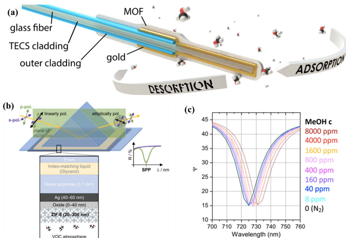
Fig. 14 (a) Schematic representation of an MOF-FO-SPR probe (not at real scale). The probe consists of an optical fibre with a diameter of 400 \mu\text{m} with the inner TECS cladding and the outer protective cladding removed from the end. A gold layer is covered with a MOF which functions as a recognition layer. The atoms in the floating methanol molecules are oxygen (red), carbon (black), and hydrogen (white). 120 (b) TIRE/SPP principle and TIRE measurement geometry with the sample layer stacks. (c) The measured SPP peak redshift in methanol compared to dry N 2 . 121
