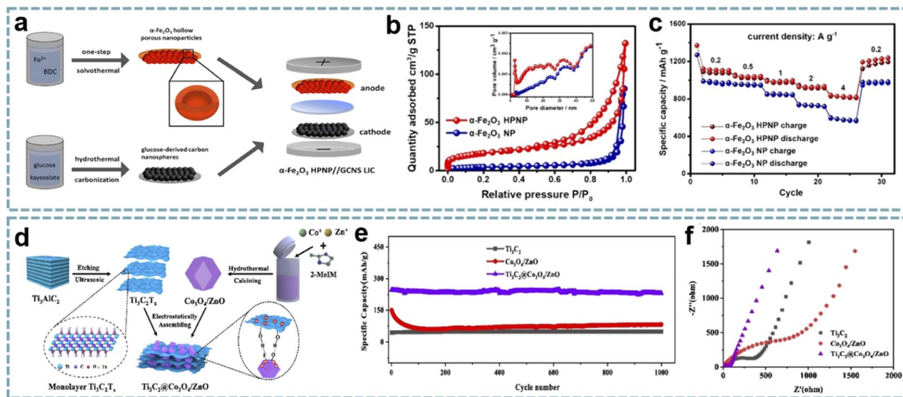
Fig. 6 MOF-derived metal compounds for MIHCs. (a) Schematic diagram of the fabrication of the \alpha -Fe 2 O 3 HPNP//GCNS LIC. (b) N 2 adsorption/desorption isotherms and pore size distributions of the \alpha -Fe 2 O 3 NP and \alpha -Fe 2 O 3 HPNP. (c) Specific capacities of the \alpha -Fe 2 O 3 NP and \alpha -Fe 2 O 3 HPNP at increasing current densities. Reproduced with permission from ref. 149. Copyright 2021, American Chemical Society. (d) Schematic diagram of the fabrication of Ti 3 C 2 @Co 3 O 4 /ZnO. (e) Cycling performance of Co 3 O 4 /ZnO, Ti 3 C 2 , and Ti 3 C 2 @Co 3 O 4 /ZnO over 1200 cycles at 2 A g -1 in a Li-half cell. (f) Nyquist plots of Co 3 O 4 /ZnO, Ti 3 C 2 , and Ti 3 C 2 @Co 3 O 4 /ZnO. Reproduced with permission from ref. 86. Copyright 2022, Elsevier.
