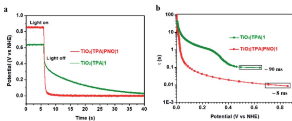
Fig. 9 (a) Open-circuit voltage decays for the electrodes \text{TiO}_2 -[TPA|PNO|1] (red) and \text{TiO}_2 |TPA|1 electrodes (green). (b) Electron lifetime derived from eqn (7) plotted as a function of V_{oc} at the transient when illumination ( >400 nm, 100 \text{ mW cm}^{-2} ) was removed. The results were obtained in 0.1 M phosphate buffer at pH 7.
