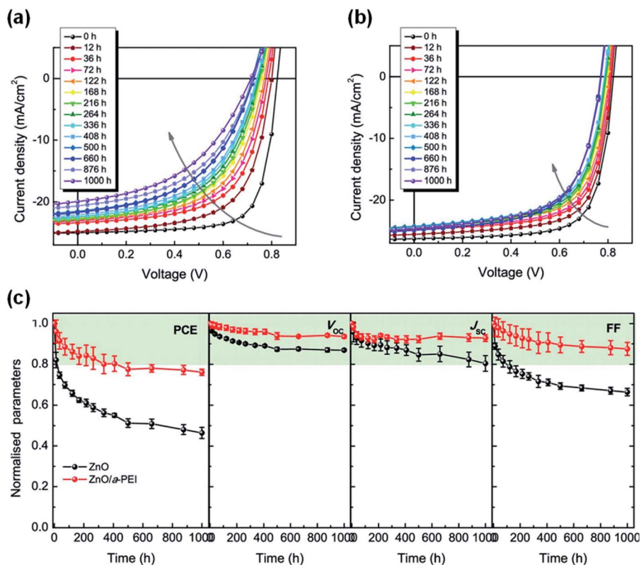
Fig. 19 Evolution of J - V characteristics under continuous AM1.5 G illumination in a nitrogen-filled glovebox with: (a) ZnO and (b) ZnO/a-PEI ETL; (c) evolution of photovoltaic parameters of the devices under continuous AM1.5 G illumination. Reproduced from ref. 49 with permission from the American Chemical Society, copyright [2021].
