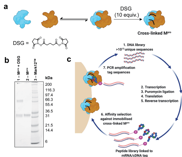
Fig. 2 (a) Scheme for cross-linking of SARS-CoV-2 M pro with disuccinimidyl glutarate (DSG). (b) SDS-PAGE gel of cross-linking reaction of M pro . Lane 1: reaction of SARS-CoV-2 M pro (25 μM) with DSG (10 equivalents relative to M pro monomer) for 1 h at 37 °C in aqueous buffer (20 mM HEPES, 100 mM NaCl, pH 7.6). Lane 2: SARS-CoV-2 M pro . Lane 3: Mark12™ ladder. (c) Workflow for the discovery of macrocyclic peptide ligands of cross-linked SARS-CoV-2 M pro using RaPID mRNA display.
