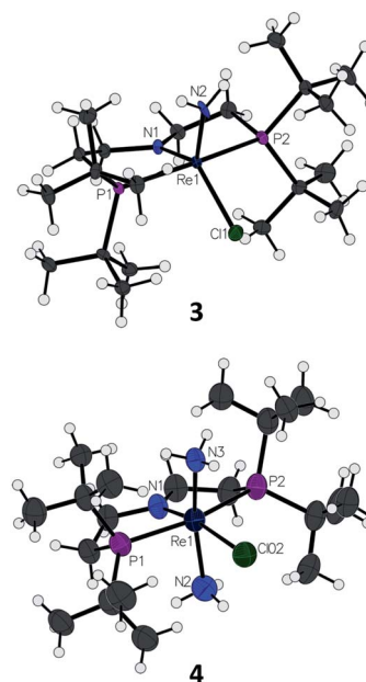
Fig. 1 Solid-state structures of \text{Re} –amide complex 3 and \text{Re}(\text{NH}_3)_2 complex 4 ( \text{BAR}^{\text{F}_4} ion omitted) with thermal ellipsoids at 50% probability.
