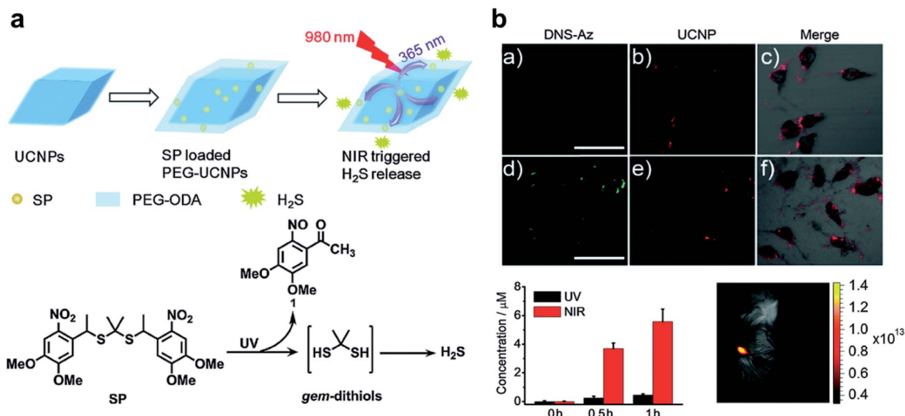
Fig. 6 UCNP-based nanocomposites for H 2 S gas therapy. (a) Construction of SP-loaded PEG-UCNPs platform for NIR-triggered H 2 S release. (b) H 2 S release from SP-loaded PEG-UCNPs with laser irradiation. 38 Adapted from ref. 38 with permission from Royal Society of Chemistry, copyright 2015.
