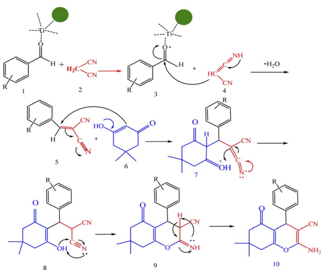
Scheme 1 A plausible mechanism for synthesis of chromens in the presence of nano-cellulose/Ti (IV) /Fe 3 O 4 .
