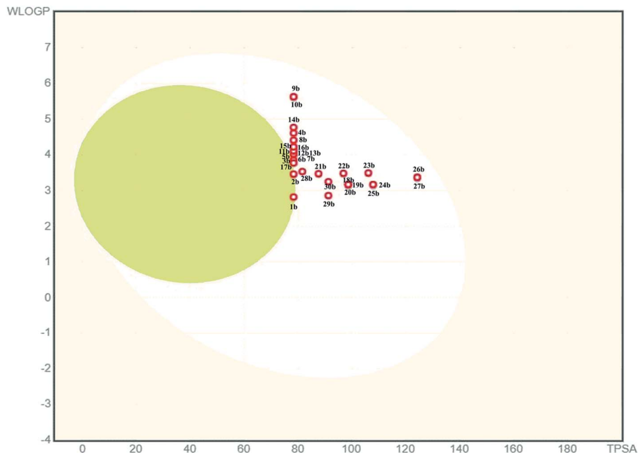
Fig. 2 Boiled egg diagram of pyridine appended 2-hydrazinylthiazoles.
