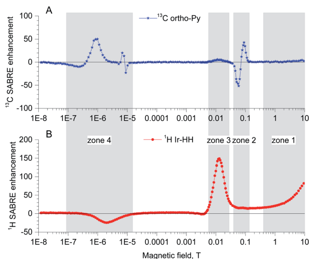
Fig. 9 (A) 13 C SABRE field dependence for ortho carbon of 15 N-pyridine, for details see ref. 142. (B) 1 H SABRE field dependence for hydride protons on Ir-catalyst (unpublished results provided by A. Kiryutin).
