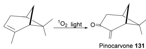
Scheme 35 Light-catalyzed oxygenation of pinene to pinocarvone.
