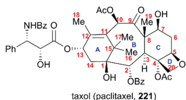
Fig. 10 The structure of taxol.
