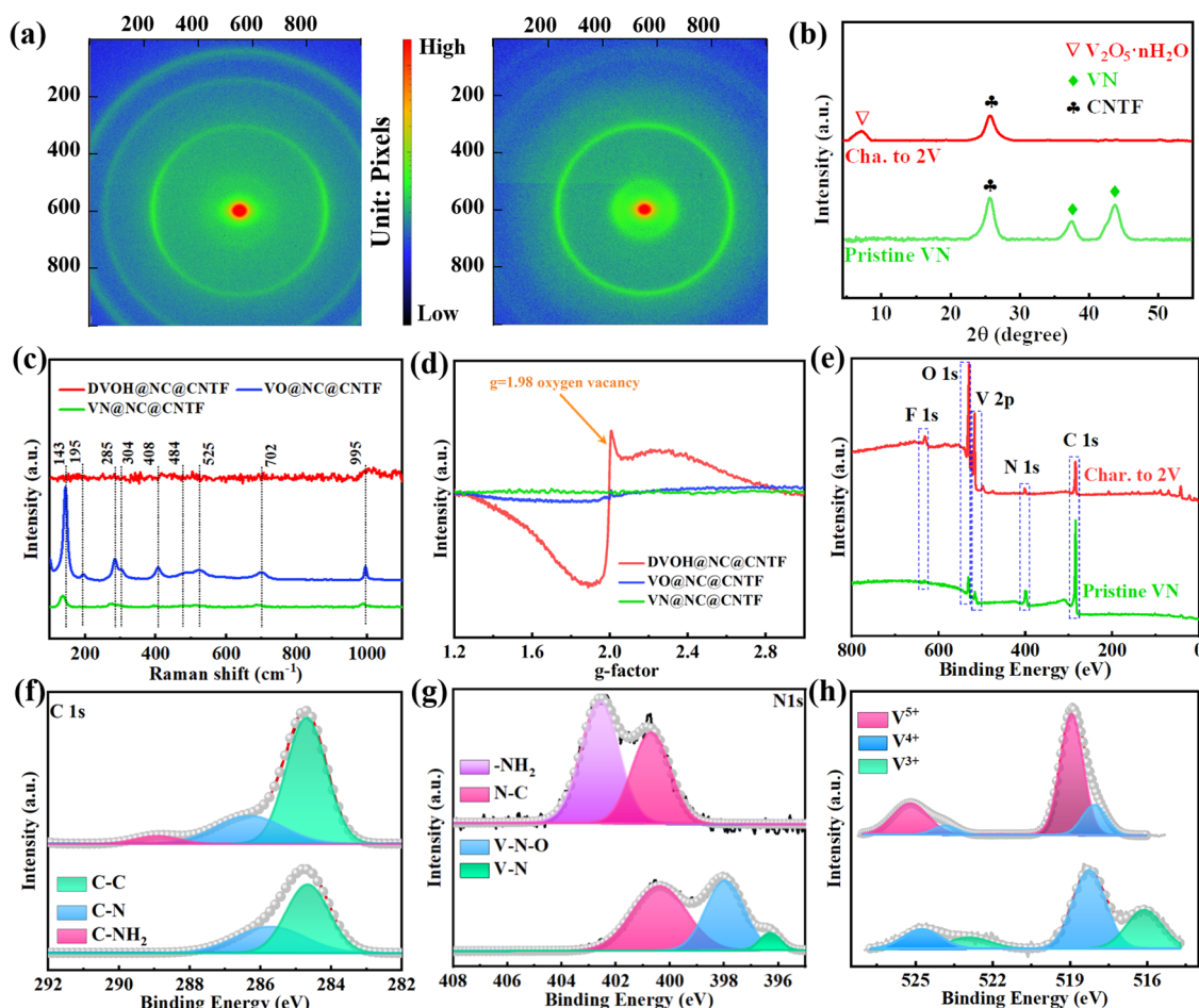
Fig. 2 (a) Transmission X-ray diffraction mapping of VN@NC@CNTF (left) and DVOH@NC@CNTF (right). (b) XRD spectra of VN@NC@CNTF and DVOH@NC@CNTF. (c) Raman spectra and (d) EPR spectra of VN@NC@CNTF, DVOH@NC@CNTF and VO@NC@CNTF. (e) Full XPS spectra and (f) C 1s, (g) N 1s and (h) V 2p high-resolution spectra of VN@NC@CNTF and DVOH@NC@CNTF.
