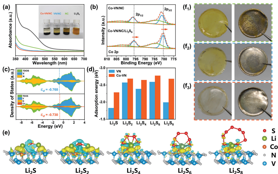
Fig. 4 (a) UV-vis spectra of Li 2 S 6 solution and ones after adding the Co-VN/NC, VN/NC and NC catalysts. Inset: Visualized adsorption test. (b) XPS Co 2 p spectrum of Co-VN/NC after Li 2 S 6 adsorption. (c) The density of states spectrum of Co-VN and VN. (d) Adsorption energy between sulfur species and Co-VN or VN on the (200) plane. (e) The optimized configurations of the Li 2 S n ( n = 1, 2, 4, 6, and 8) molecules adsorbed on the surface of Co-VN. Photographs of the separators and lithium foils in the NC (f 1 ), VN/NC (f 2 ) and Co-VN/NC (f 3 ) cells.
