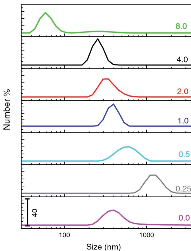
Fig. 3 Particle size distribution of ZnO samples synthesized using various concentrations of UR (g); 0, 0.25, 0.5, 1, 2, 4, and 8 (w/w%) (reproduced from ref. 84 with permission from Springer).
