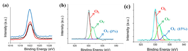
Fig. 6 (a) Zn 2p XPS spectra peaks of ZNLs and ZNWs, (b) O 1s XPS spectra of ZNLs, and (c) O 1s XPS spectra of ZNLs.
