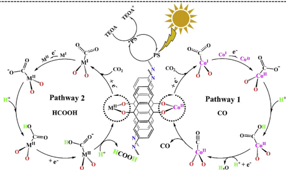
Fig. 7 Synthesis and metallization process of DQTP COF and DATP COF and proposed mechanism for the photocatalytic reduction of CO 2 with DQTP-COF-M (M = Zn, Ni, and Co). Adapted from ref. 107. © 2019 Elsevier B.V. All rights reserved.
