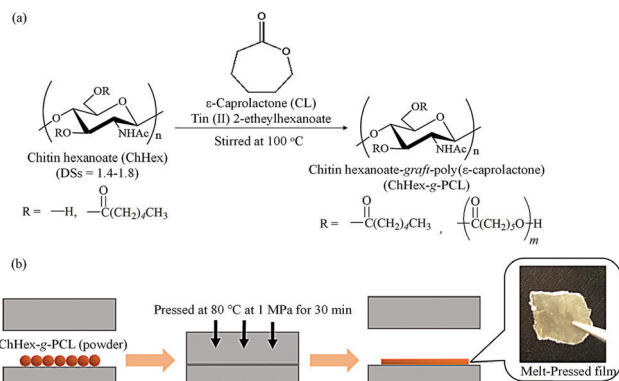
Fig. 14 (a) Surface-initiated ring-opening graft polymerization of \epsilon -caprolactone (CL) from chitin hexanoates (ChHex) to obtain chitin hexanoate- graft -poly( \epsilon -caprolactone) (ChHex- g -PCL), and (b) melt-pressing experiment of ChHex- g -PCL (reprinted with permission from ref. 121. Copyright 2022 Elsevier; DOI: 10.1016/j.carbpol.2021.119024).
