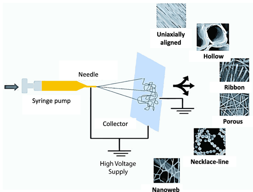
Fig. 3 Schematic setup for electrospinning and different morphologies of electrospun polymeric fibers. Adapted from ref. 53 with permission from the Royal Society of Chemistry.
