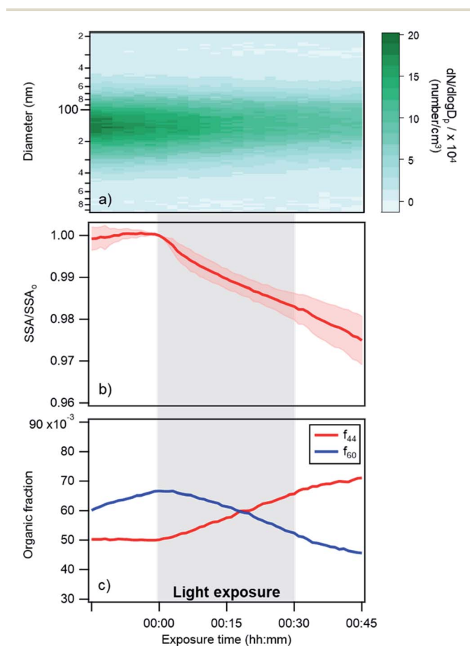
Fig. 3 Changes in (a) particle size distribution, (b) single scattering albedo at 405 nm, and (c) AMS f_{44} and f_{60} fractions over time for a typical photoreaction experiment in dry conditions. Darker shaded regions in panel (a) represent a higher number concentration of particles. In panel (b) the SSA is represented as the ratio of experimental SSA over the SSA at exposure time = 0, in order to directly compare different experiments. The shaded pink region in (b) represent the standard deviation (for 4 different replicates). Note that the changes in f_{44} and f_{60} during a control experiment (Fig. S4†) were much smaller than the changes shown in this figure; (a) and (c) are results for one replicate.
