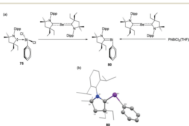
Fig. 26 (a) Synthesis of carbene-stabilized bismuthinidene compound 80 , (b) solid-state structure of 80 .
