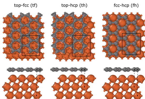
Fig. 1 Graphene binding to the Fe fcc(111) surface in three different configurations: top–fcc (tf), top–hcp (th), and fcc–hcp (fh). The black rectangle in the periodic image represents the applied cells in the computations.
