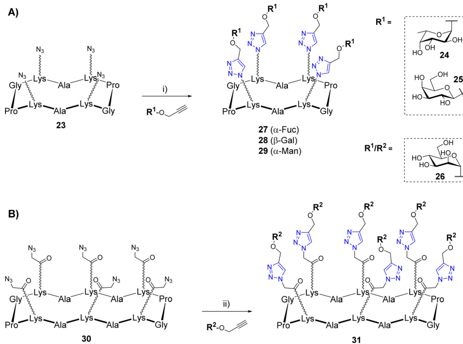
Scheme 4 Assembly of glycoclusters by CuAAC: (A) from the tetravalent scaffold 23 ; (B) from the hexavalent scaffold 30 . Reagents and conditions: (i) Cu micropowder, tBuOH/ACONH 4 (pH 7.4), r.t., 3 h, 70–75%; (ii) CuSO 4 ·5H 2 O, THPTA, sodium ascorbate, PBS (pH 7.4), r.t., 1 h, 85%.
