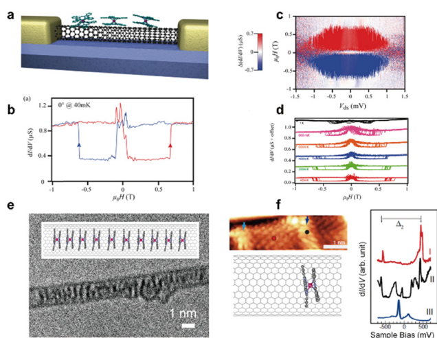
Fig. 35 Supramolecular spin valves based on the \text{Tb(Pc)}_2 -SWCNT hybrid device. (a) Schematic illustration of the device. (b) Conductance hysteresis loops of \text{Tb(Pc)}_2 -SWCNT. dI/dV measured at 40 mK with an in-plane magnetic field applied along the easy axial direction ( 0^\circ ). Bias and temperature dependences of the conductance hysteresis loops of \text{Tb(Pc)}_2 -SWCNT. (c) Scale map of the dI/dV hysteresis as a function of the in-plane magnetic field and source drain voltage ( V_{ds} ). (d) Temperature dependence of the conductance hysteresis loops. (e) Supramolecular structure of the \text{Tb(Pc)}_2\text{@SWCNT} hybrid material. TEM image and schematic illustration of \text{Tb(Pc)}_2\text{@SWCNT} . (f) STM image showing empty (red dot) and filled (black dot) regions. Comparative STS spectra measured at the red and black dotted points in STM image. The STS of \text{Tb(Pc)}_2 adsorbed on an Au(111) surface is illustrated as plot III (blue) in (f) as a reference. Reprinted from (a–d) ref. 269. Copyright 2011, MDPI. Reproduced from (e and f) ref. 422. Copyright 2021, Royal Society of Chemistry.
