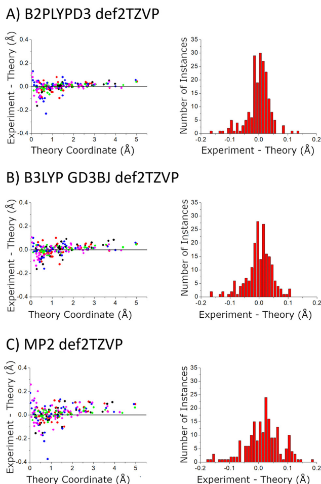
Fig. 9 The accuracy of the quantum chemistry structures is benchmarked using the carbon atom coordinates – in the principal axis system for molecular rotation – obtained from the Kraitchman analysis. The scatter plot shows the difference in the absolute values of these coordinates (coordinate signs are unavailable from the spectroscopic analysis) as a function of the size of the coordinate. The coordinates come from the 5 structures that were measured with ^{13}\text{C} -sensitivity; HOMEC2D1 (black), HOMBC2D1 (blue), HOMBC1D1 (magenta), HETEC1D1 (red), and HETBC1D1 (green). The figure for calculations with the 6-311++G(d,p) basis set is shown in the ESI.†
