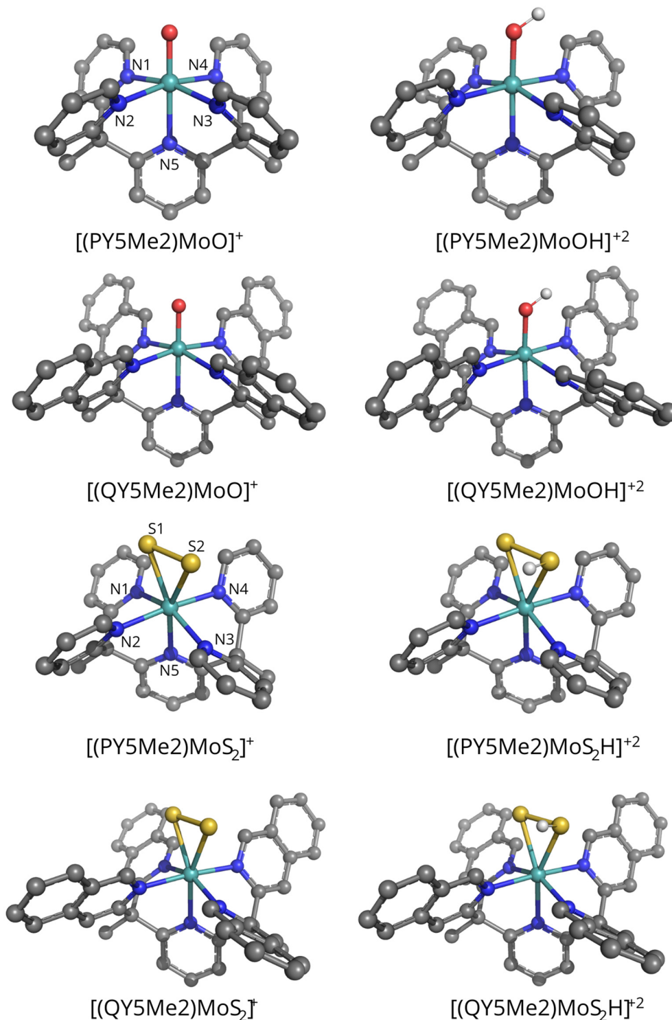
Fig. 2 Representation of the vacuum-optimized structures of the [(PY5Me_2)MoO]^+ , [(QY5Me_2)MoO]^+ , [(PY5Me_2)MoS_2]^+ and [(QY5Me_2)MoS_2]^+ catalysts and of their respective protonated products ( [(PY5Me_2)MoOH]^{+2} and [(QY5Me_2)MoOH]^{+2} , [(PY5Me_2)MoS_2H]^{+2} and [(QY5Me_2)MoS_2H]^{+2} ). Colour code: Mo, cyan; S, yellow; O, red; N, blue; C, grey; H, white.
