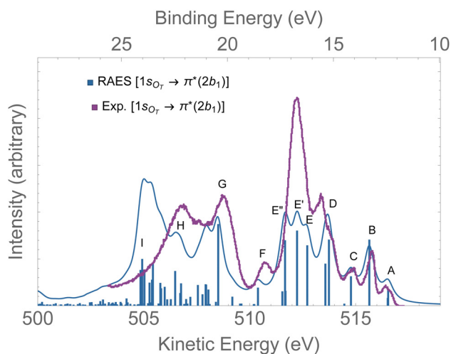
Fig. 4 RAES of O_3 at the 1s_{O_T} \rightarrow \pi^*(2b_1) resonance calculated with the FC geometry. The computed spectrum was shifted by -0.6 \text{ eV} and broadened with Lorentzian functions with fwhm = 0.30 eV. The experimental spectrum was digitized from ref. 12. For the assignments, see Table 1.
