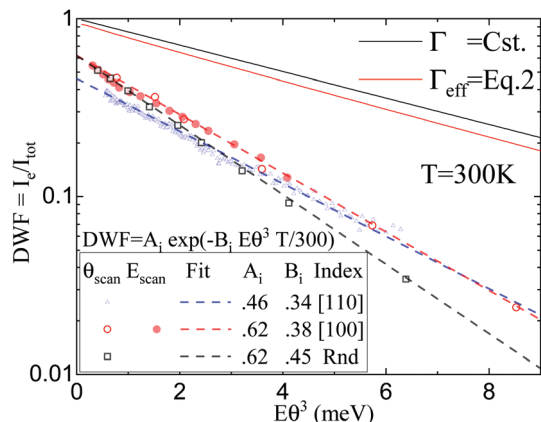
Fig. 7 The \text{DWF} = \frac{I_e}{I_{\text{tot}}} from 3 LiF samples are reported as a function of E\theta^3 . The dotted lines are fits to the data while the solid lines are numerical prediction of eqn (1) with (red A = 0.94 , B = 0.19 ) and without corrections (black A = 1 , B = 0.17 ) due to the attraction towards the surface.
