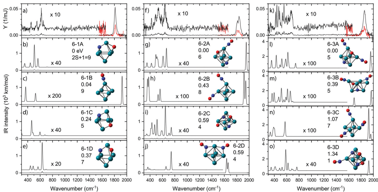
Fig. 8 IR-MPD spectra for \text{Rh}_6^+(\text{NO})_m, \text{Ar} (panels a, f, k) recorded at full (black traces) and reduced (red) IR laser power, accompanied by unscaled harmonic spectra calculated at the B3LYP/sdd/aug-cc-pVDZ level. The associated cluster structures are accompanied by the energy relative to the most stable species, and spin multiplicity. Rh, N, and O atoms are depicted using green, blue, and red spheres, respectively. Data from ref. 91 and 109.
