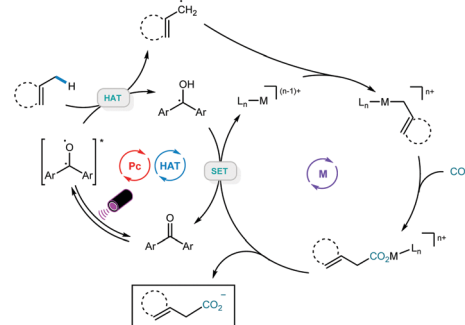
Scheme 19 Photoredox and copper/nickel dual-catalyzed benzylic and allylic C(sp^3) –H carboxylation.
