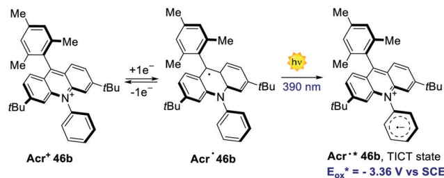
Scheme 39 The strongly reducing radical Acr^{\bullet\bullet+} 46b , formed upon the excitation of the acridium radical Acr^+ 46b .
