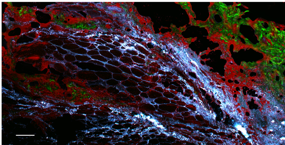
Fig. 7 SRS and SHG microscopy composite image of a rat skin section containing metallic particles. SRS contrast for \text{CH}_2 stretching at 2850 \text{ cm}^{-1} is shown in red, and off-resonance signals at 2770 \text{ cm}^{-1} are overlaid in cyan hot, revealing the distribution of the metal particles based on their strong signals due to absorption and photothermal lensing. Collagen (green) is visualised using SHG. The scale bar represents 100 \mu\text{m} .
